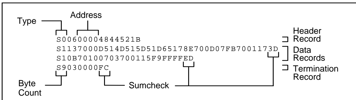
Figure 10.5: Motorola S Format
