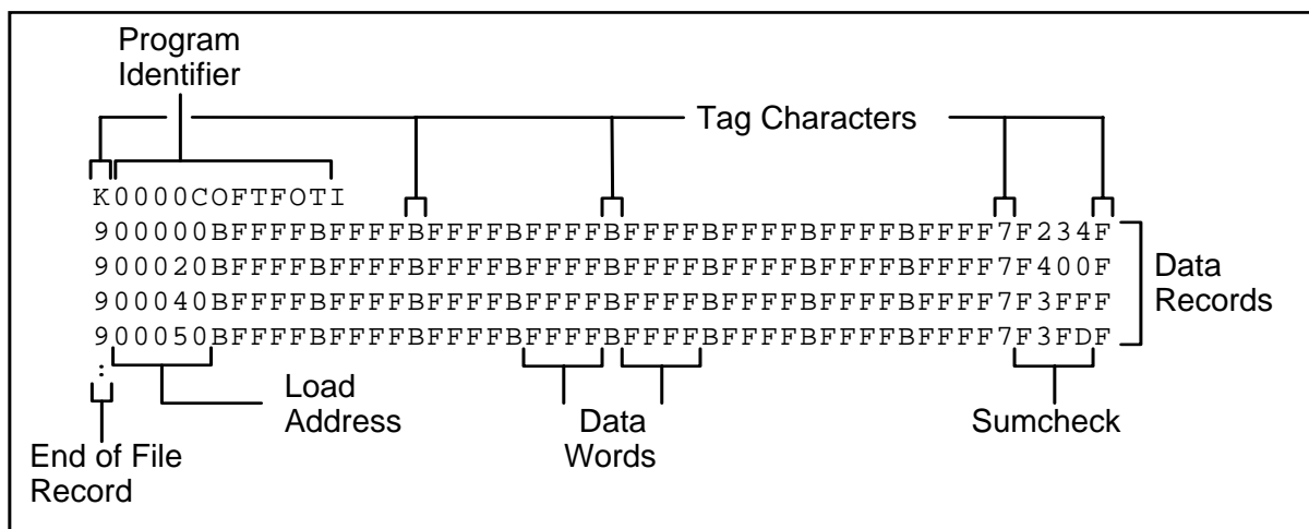
Figure 10.4: TI-Tagged Object Format
