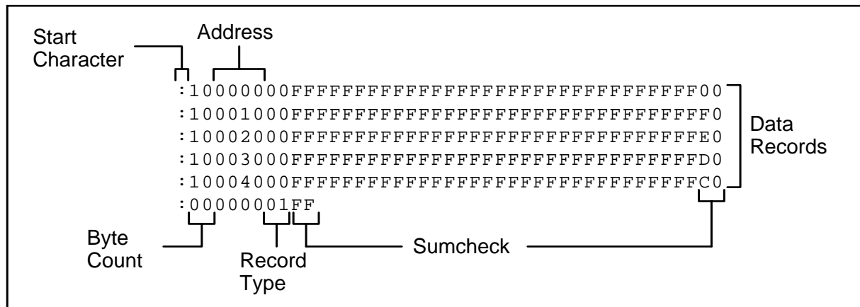
Figure 10.3: Intel Hex Object Format
