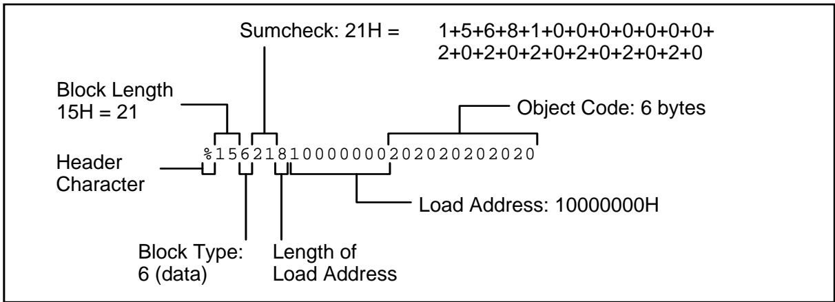
Figure 10.2: Extended Tektronix Hex Object Format
