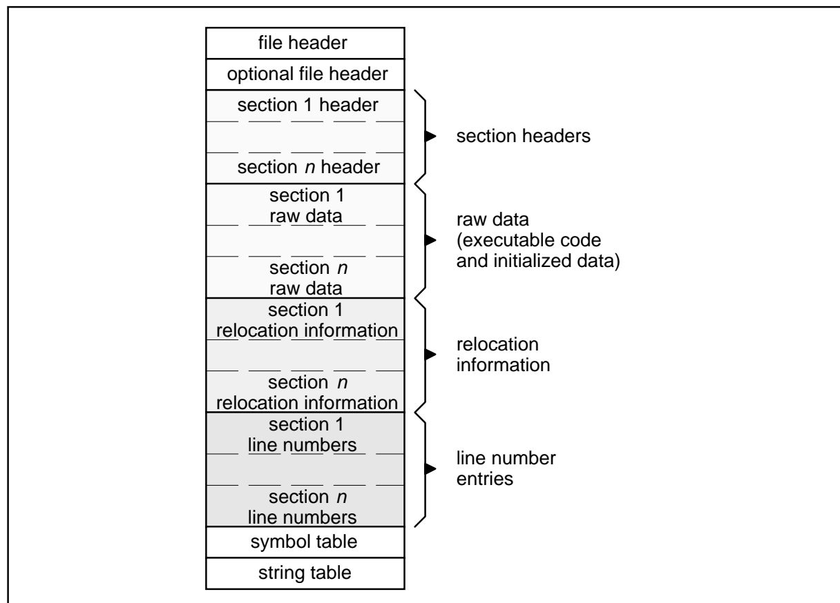
Figure 20.1: COFF File Structure
