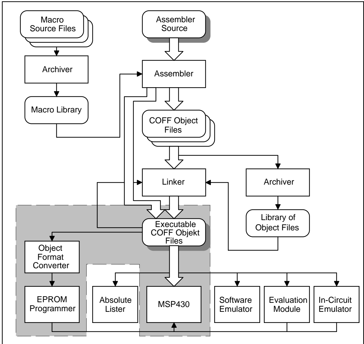
Figure 10.1: Object Format Converter Development Flow
