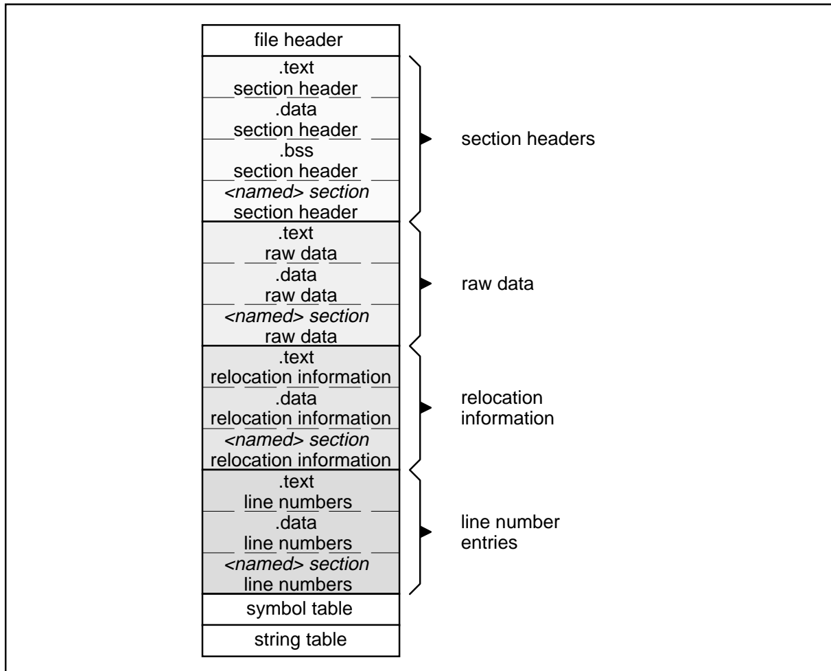
Figure 20.2: Sample COFF Object File
